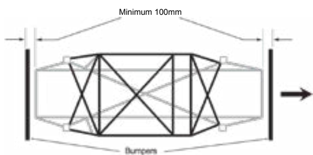
Drawing.8.5 Plan view
